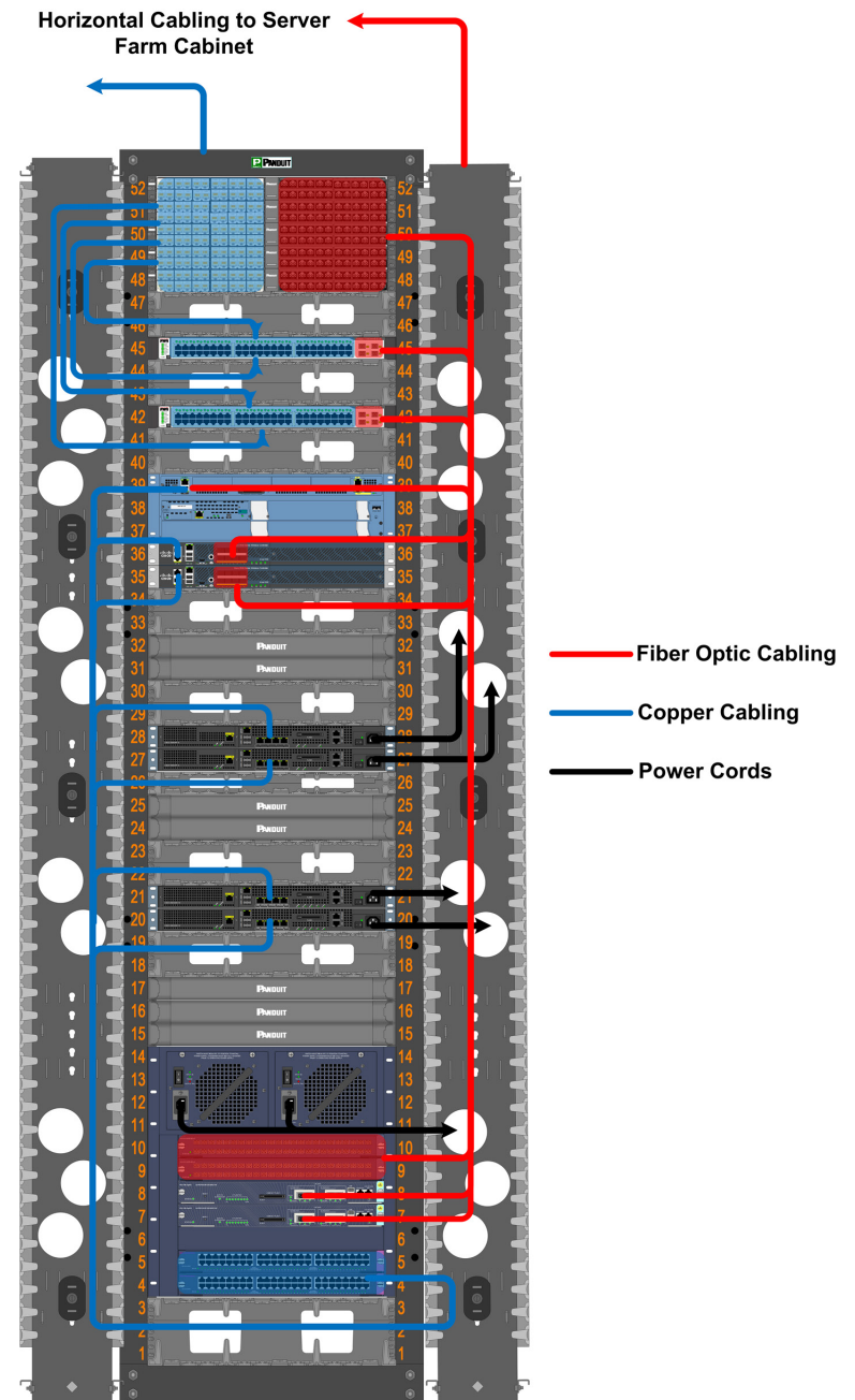
Figure 7 - Cable routing within R1
